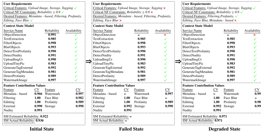
Fig. 7. Initial, failed, and degraded state of the service composition in Fig. 4 after failure of the Object Detection service.
