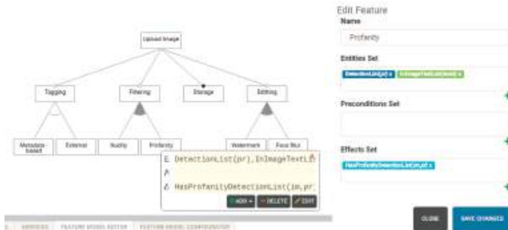
Fig. 12. The Domain Design Tool interface for annotating features in the feature model.
