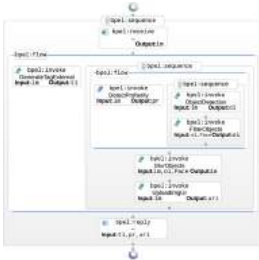
Fig. 10. BPEL process visualization for an alternate solution for BPEL process in Fig. 4 after adaptation by feature model reconfiguration as a result of the decrease in the reliability of the ObjectDetection service.
