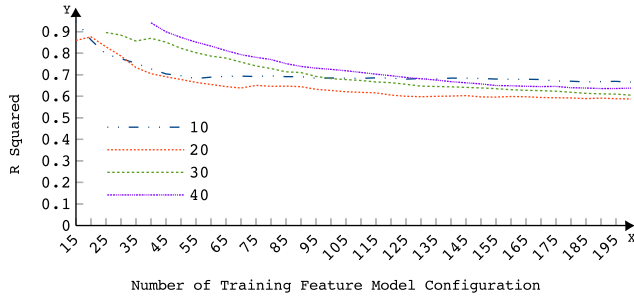
Fig. 19. R Squared of regression model for estimation in terms of number of training feature model configuration.
