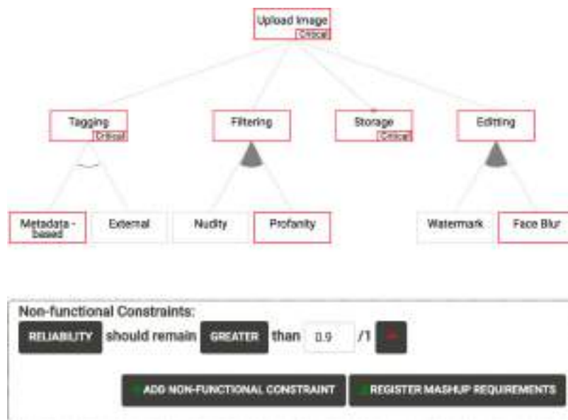
Fig. 13. The Configuration Tool interface for specifying user's requirements.
