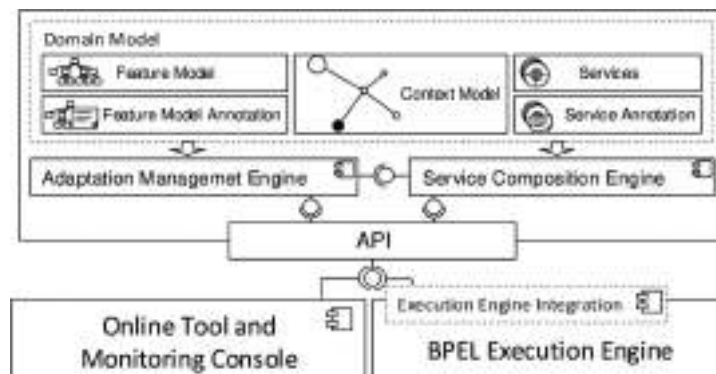
Fig. 11. Architecture of the proposed method.
