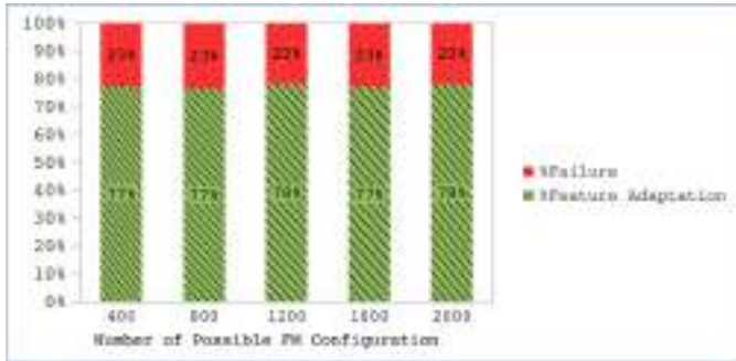
Fig. 16. Distribution of success versus failure of the adaptation mechanism.
