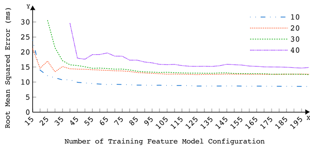
Fig. 20. Root Mean Squared Error of the estimation method in terms of number of training feature model configuration.
