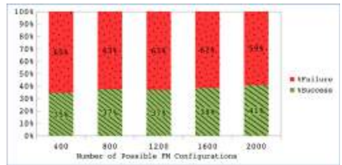
Fig. 21. Distribution of success versus failure mechanisms after a non-functional constraint violation.
