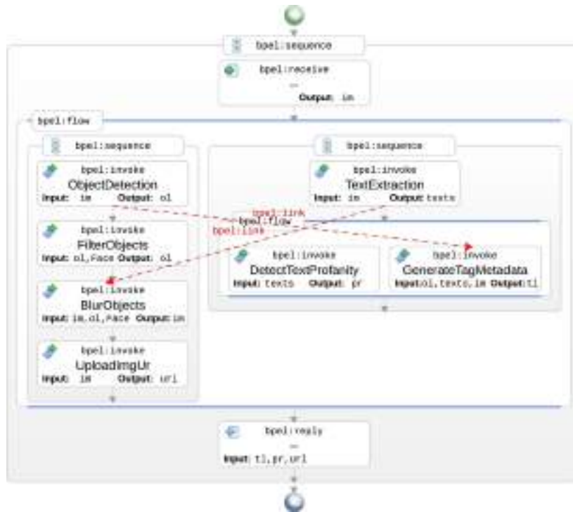
Fig. 4. BPEL process visualization for a possible service composition satisfying requirements of the feature model configuration in Fig. 1.
