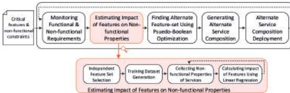
Fig. 5. General overview of the proposed approach for self-healing from functional and non-functional failure.
