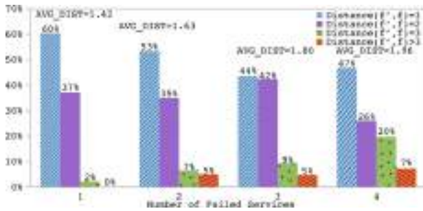
Fig. 18. Distribution of the distance between the alternate feature model configuration and the failed one after service failure in terms of number of failed services.
