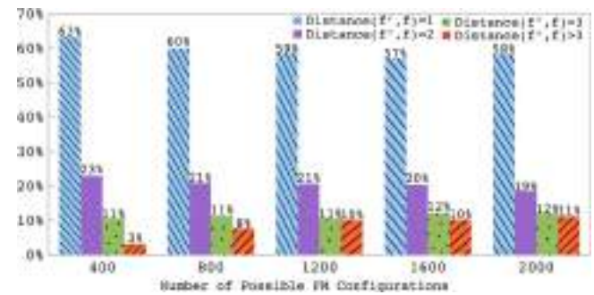
Fig. 22. The distribution of the distance between the alternate feature model configuration and the failed one after a non-functional constraint violation.
