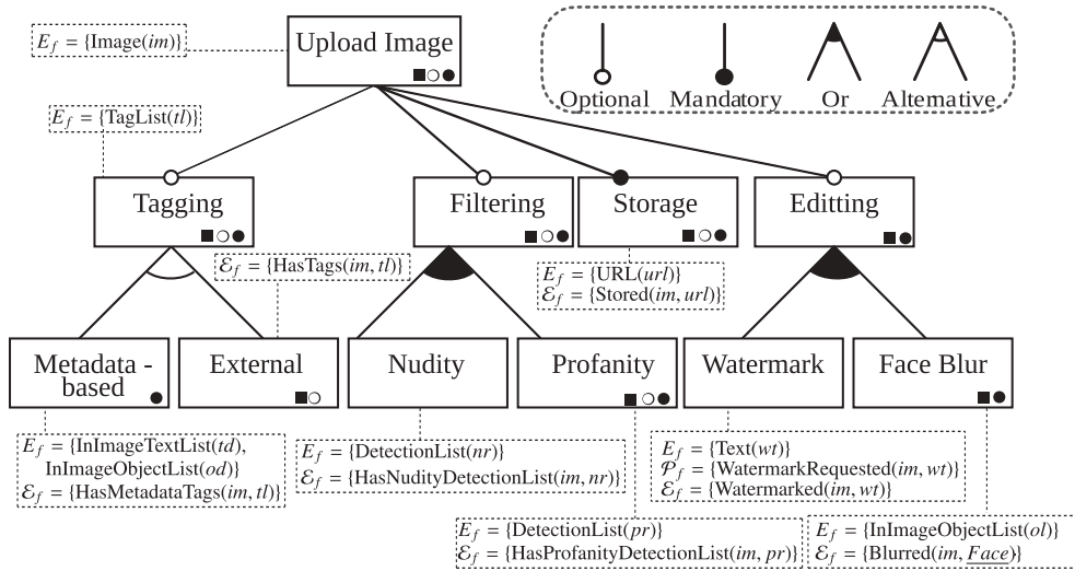
Fig. 1. An annotated feature model for the upload image service family.
