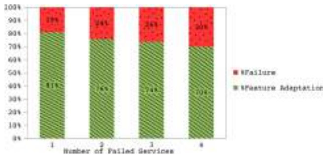
Fig. 17. Distribution of success versus failure mechanisms after a service failure in terms of number of failed services.
