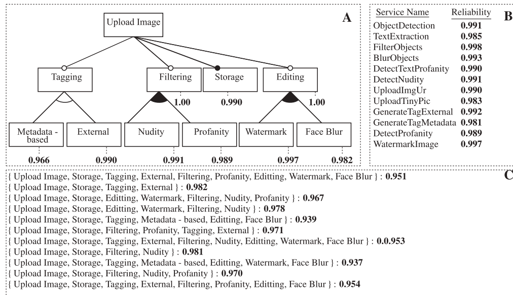
Fig. 6. A. Feature model annotated with contribution value of each feature to the reliability of the service composition. B. Reliability of the individual services in the service family C. An example of a dataset used for estimating the contribution value of each feature to the reliability of the service composition.
